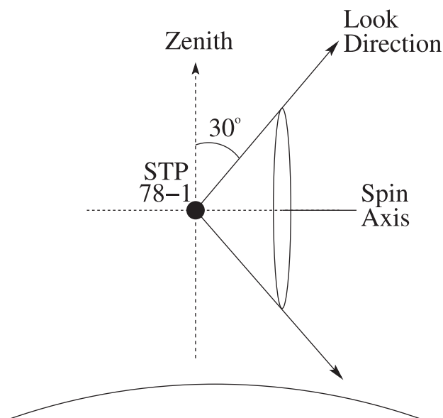
Figure 1. Schematic showing the cone swept out by the field of view of the spectrograph on the STP78-1 satellite. The satellite orbital motion is normal to the plane of the figure. This configuration assures the spectrograph will not look closer than 30^\circ to the Sun.
