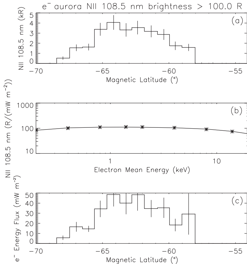
Figure 11. (a) Observed N II 108.5-nm brightness as a function of magnetic latitude, after removal of the proton contribution. (b) Modeled N II 108.5-nm brightness as a function of electron mean energy. The distribution in energy of the incident electrons is assumed to be a Maxwellian with a low-energy tail. The energy flux is normalized to 1 mW m -2 . The stars are results of several simulations and the solid line is a fit to these points. (c) Estimated electron energy flux as a function of magnetic latitude. The energy flux is inferred only where the observed N II 108.5-nm total brightness (after removal of the proton contribution) is larger than 100 R. The error bars in (a)–(c) are associated with the uncertainties in the measured brightnesses. This includes both statistical and calibration uncertainties. They represent the standard variation ( \pm 1 \sigma ).
