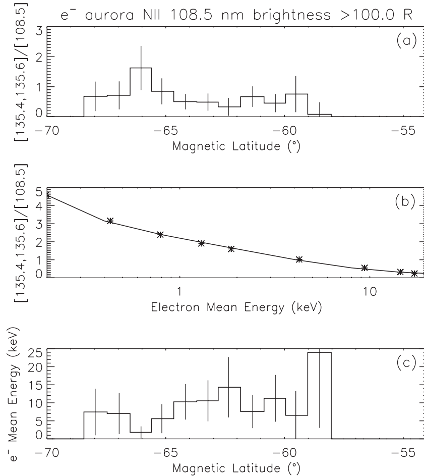
Figure 10. (a) Observed brightness ratio of (N 2 135.4 nm, O I 135.6 nm) to N II 108.5 nm as a function of magnetic latitude, after removal of the proton contribution. (b) Modeled brightness ratio of (N 2 135.4 nm, O I 135.6 nm) to 108.5 nm as a function of electron mean energy. The distribution in energy of the incident electrons is assumed to be a Maxwellian with a low energy tail. The stars are results of several simulations and the solid line is a fit to these points. (c) Estimated electron mean energy as a function of magnetic latitude. The mean energy is inferred only where the observed N II 108.5 nm total brightness (after removal of the proton contribution) is larger than 100 R. The error bars in (a–c) are associated with the uncertainties in the measured brightnesses and include both statistical and calibration uncertainties. They represent the standard variation ( \pm 1 \sigma ).
