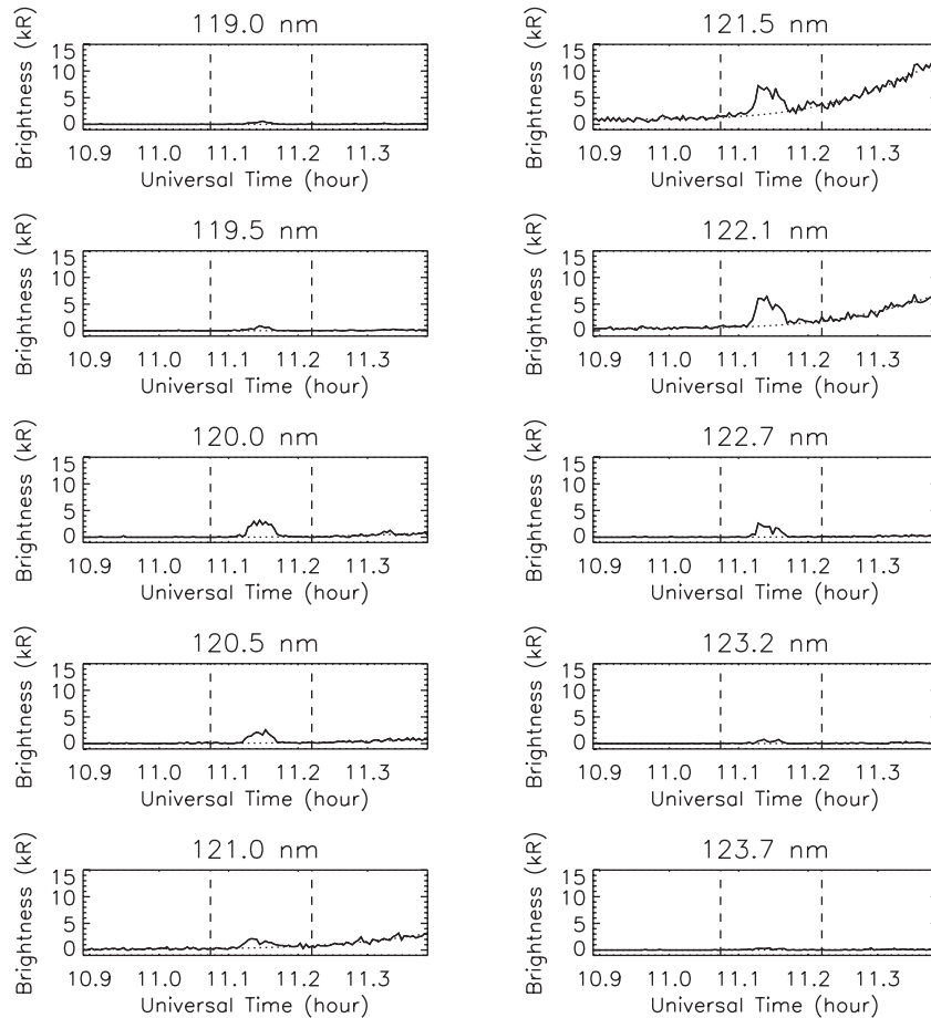
Figure 4. Geocoronal component (dotted line) and total signal (solid line) shown for 10 wavelength bins, each covering a \sim 0.5 nm band for the A1 region (dotted box in Figure 3). The estimation of the geocoronal background is based on a fit to the signal outside the auroral zone and on an interpolation within the auroral zone defined as the region within the dashed vertical line.
