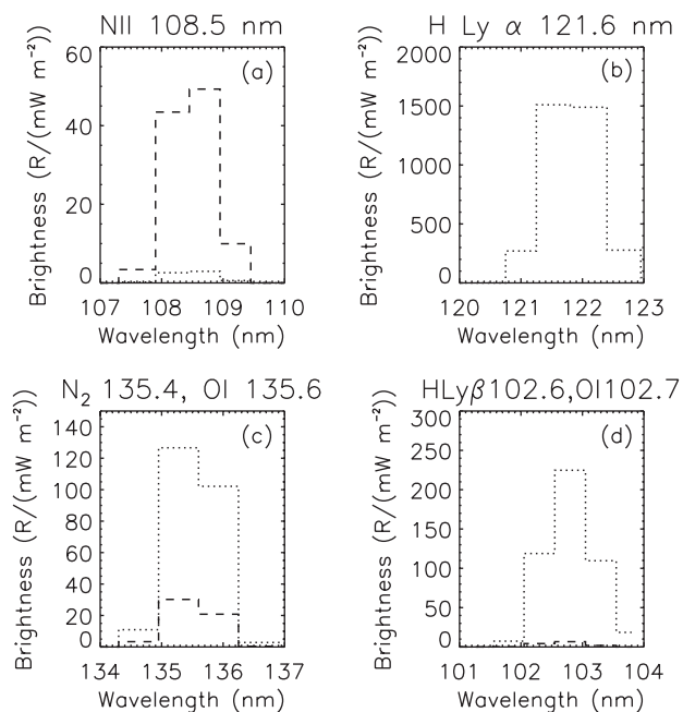
Figure 8. Modeled spectra for different emissions induced by energetic protons (dotted lines) and electrons (dashed lines) binned to the instrument resolution. These spectra have been obtained after convolution of the modeled emission yield (or Doppler profile, for H emissions) with the instrumental function assumed to be triangular with a FWHM of 0.8 nm. The satellite viewing direction considered is 30^\circ from nadir. The distribution in energy of the incident particles is a Maxwellian with, for the electrons, a low energy tail. The mean energies assumed for electrons and for protons are 8 and 30 keV, respectively.
