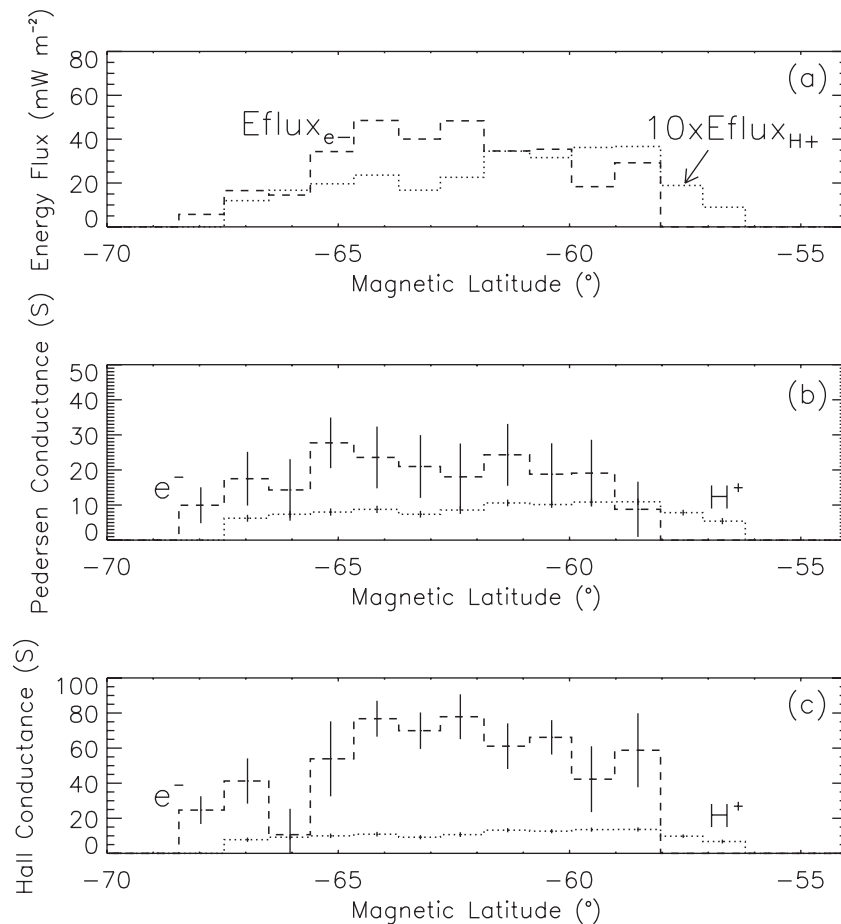
Figure 13. Estimated parameters derived from the analysis of STP78-1 FUV spectra for electron aurora (dashed line) and for proton aurora (dotted line): (a) Particle energy flux (note that the dotted line shows the proton energy flux multiplied by 10); (b) Pedersen conductance; (c) Hall conductance. The error bars are associated with the uncertainties in the measured brightnesses. This includes both statistical and calibration uncertainties. They represent the standard variation ( \pm 1 \sigma ).
