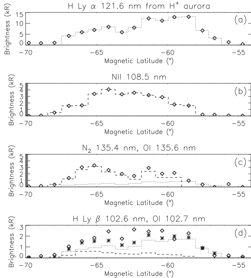
Figure 12. Observed (diamond) and modeled electron-induced (dashed line) and proton-induced (dotted line) brightnesses as a function of magnetic latitude for different auroral emissions: (a) H Ly \alpha produced only in proton aurora; (b) N II 108.5 nm; (c) N 2 135.4 nm and O I 135.6 nm; (d) H Ly \beta and O I 102.7 nm. The stars represent the modeled brightness from both electron and proton aurora.
