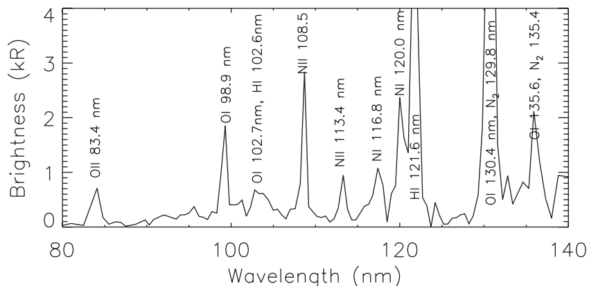
Figure 2. FUV spectrum observed at a magnetic latitude of -63^\circ by STP78-1.
