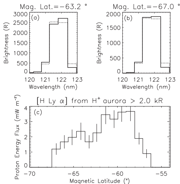
Figure 9. (a and b) Spectra in the vicinity of H Ly \alpha for two different magnetic latitudes, (left) at -63.2^\circ and (right) at -67.0^\circ . The observed spectra obtained after removal of the geocoronal background are shown with solid lines. The modeled spectra are shown as dotted lines. (c) Estimated proton energy flux as a function of magnetic latitude. The energy flux is inferred only where the observed H Ly \alpha total brightness - after removal of the geocoronal background - is larger than 2 kR. The error bars are associated with the uncertainties in the measured brightnesses and include both statistical and calibration uncertainties. They represent the standard variation ( \pm 1 \sigma ).
