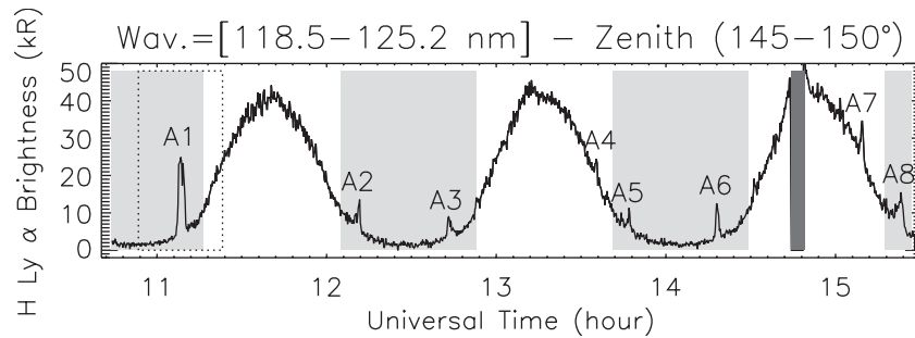
Figure 3. Spectra H Ly \alpha brightness over three orbits of STP78-1 during 22 March 1979 is shown as a function of universal time (UT). The shaded stripes correspond to a solar zenith angle larger than 90^\circ . The black strip at 1445 UT is associated with a time period during which no data were acquired. The smooth, sinusoidal variation is produced by sunlight scattering in the geocorona. The sharp peaks (A1 to A8) correspond to the proton aurora. The A1 region analyzed in this paper is delimited by the dotted box.
