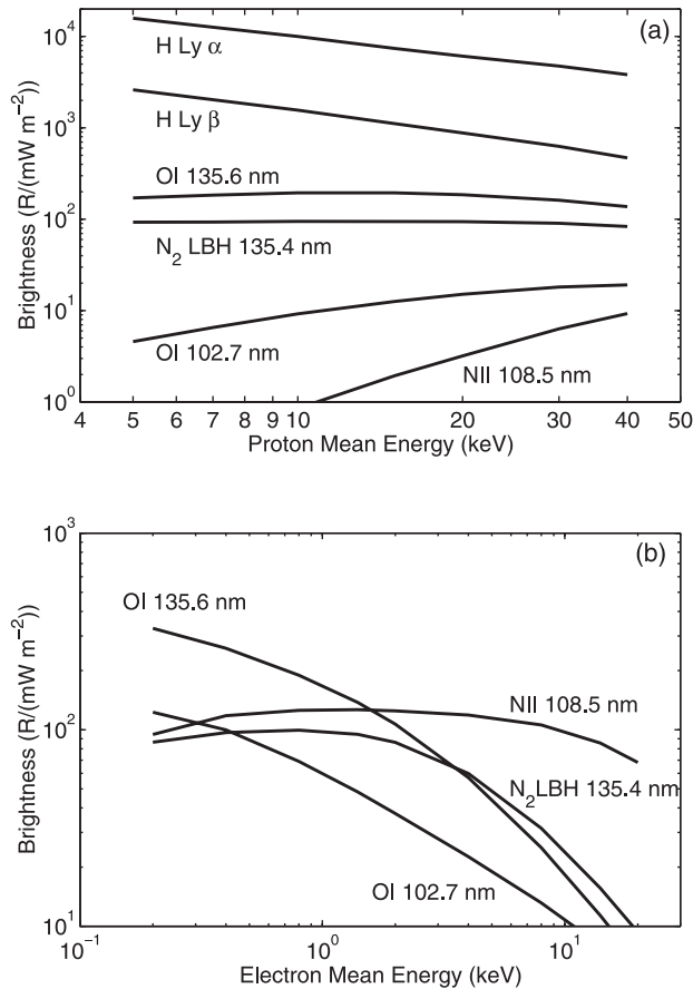
Figure 7. (a) Modeled emission yields as a function of the mean energy of the incident protons. The distribution in energy is assumed to be a Maxwellian with a normalized energy flux of 1 \text{ mW m}^{-2} . The satellite viewing direction considered is 30^\circ from nadir. (b) The same as the top panel, but for electrons. Note that the distribution in energy for electrons is a Maxwellian with a low-energy tail.
