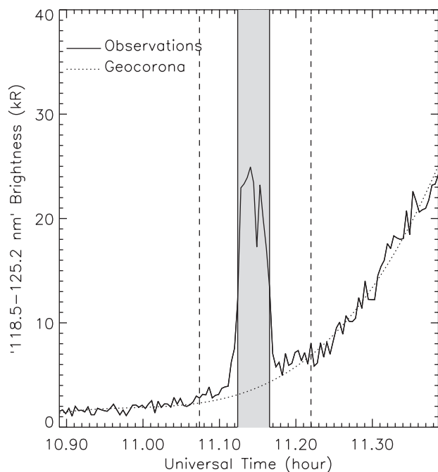
Figure 5. Total (solid line) and inferred geocoronal (dotted) brightnesses, integrated between 118.5 and 125.2 nm, as a function of universal time for the A1 region (dotted box in Figure 3). The dashed vertical lines delimit the auroral zone considered for estimating the geocoronal component (cf. Figure 4). The shaded box defines a region of strong proton aurora spreading over magnetic latitudes from -67.0^\circ to -57.5^\circ . Within this region the contribution from the geocoronal background is between 14 and 32% of the observed HI brightness.
