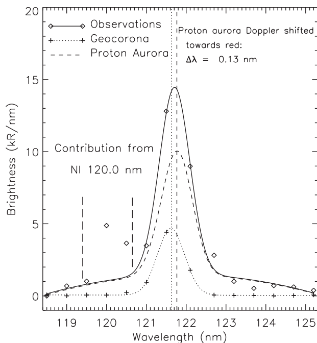
Figure 6. Spectral profiles, in the vicinity of HI 121.6 nm, of the observed signal (solid line) and geocoronal background (dotted line) to the binned data, represented with diamonds and crosses, respectively. The brightnesses have been averaged over the strong proton aurora region (shaded box in Figure 5). Note that the fitting process disregards the three bins in the neighborhood of N I 120.0 nm. The dashed line shows the contribution from the proton aurora derived from the two other profiles. As expected, the geocoronal profile is centered at the rest wavelength H I 121.6 nm (vertical dotted line), whereas the proton aurora profile is Doppler-shifted toward the red (vertical dashed line).
