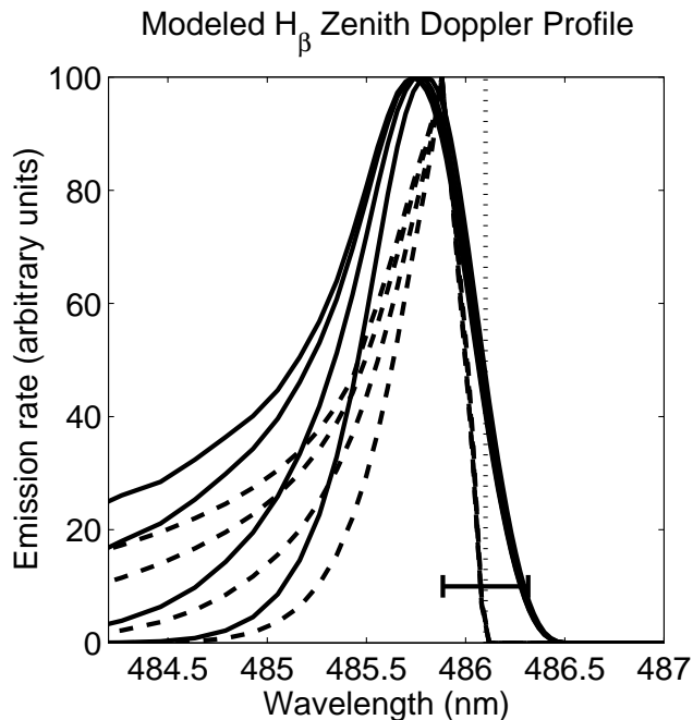
Figure 1. H_{\beta} line profiles from model calculations without angular redistribution for incident Maxwellian proton spectra with E_0 of 1, 3, 10, and 20 keV. The dashed lines are the emission Doppler profiles; the solid lines are the same profiles convolved with an instrument function with full width at half maximum (FWHM) of 0.43 nm. The dotted vertical line indicates the unshifted emission wavelength (486.1 nm); the horizontal bar shows the instrument FWHM. Each profile is normalized for comparison. The blue wing of the line profile brightens as E_0 increases.
