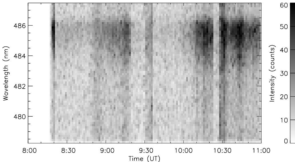
Figure 3. Spectrograms of H_{\beta} for March 21, 1998, obtained by averaging five scans for a time resolution of 80 s. Brightness is in uncalibrated counts. A co-located meridian scanning photometer (MSP) indicated H_{\beta} of up to 100 R at \sim 1045 UT.
